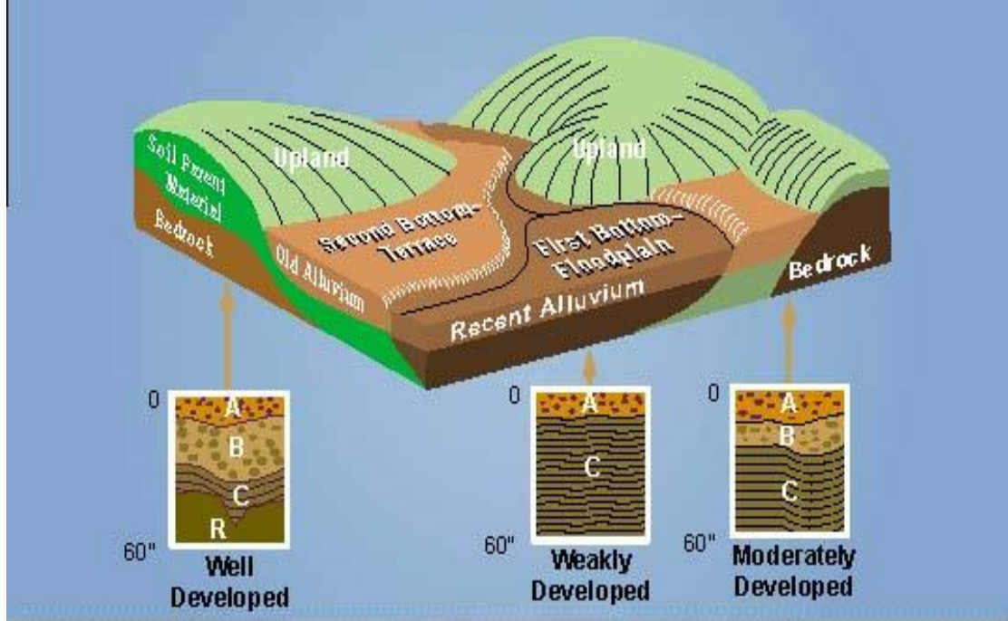
Landscape position, climate, time, organisms, and parent materials influence soil development.
